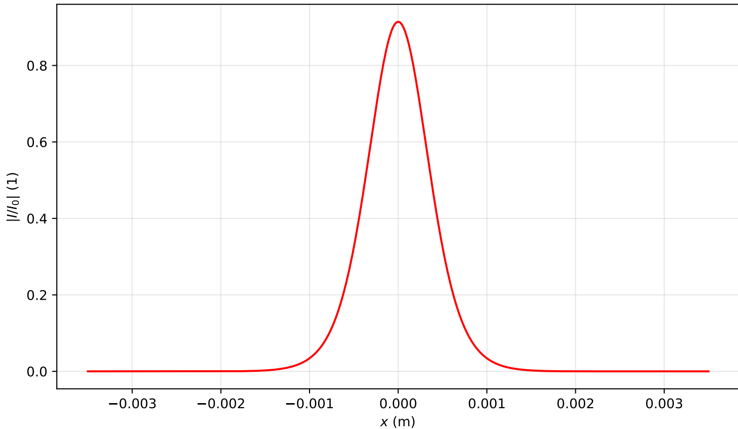
Intensity profile I(x, y = 0, z = 1.672)/I_0 , P_{in}=0.5P_{cr} , artificial time
